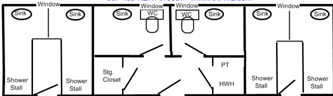
ATCO Type Building 40' x 10' on Skids Not to Scale Unit Nickname "Coldfoot"
