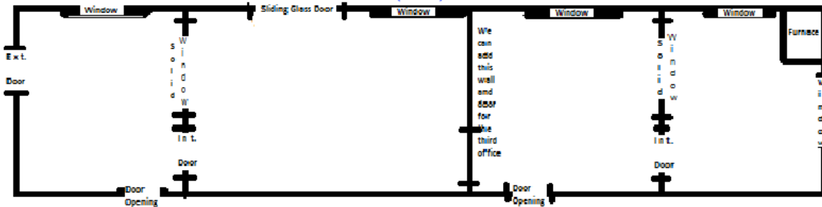
ATCO 50 x 10 +/- 2 (or 3) Offices plus Reception Area with furnace - on skids Not to scale Unit Nickname: "Atigun Pass"
